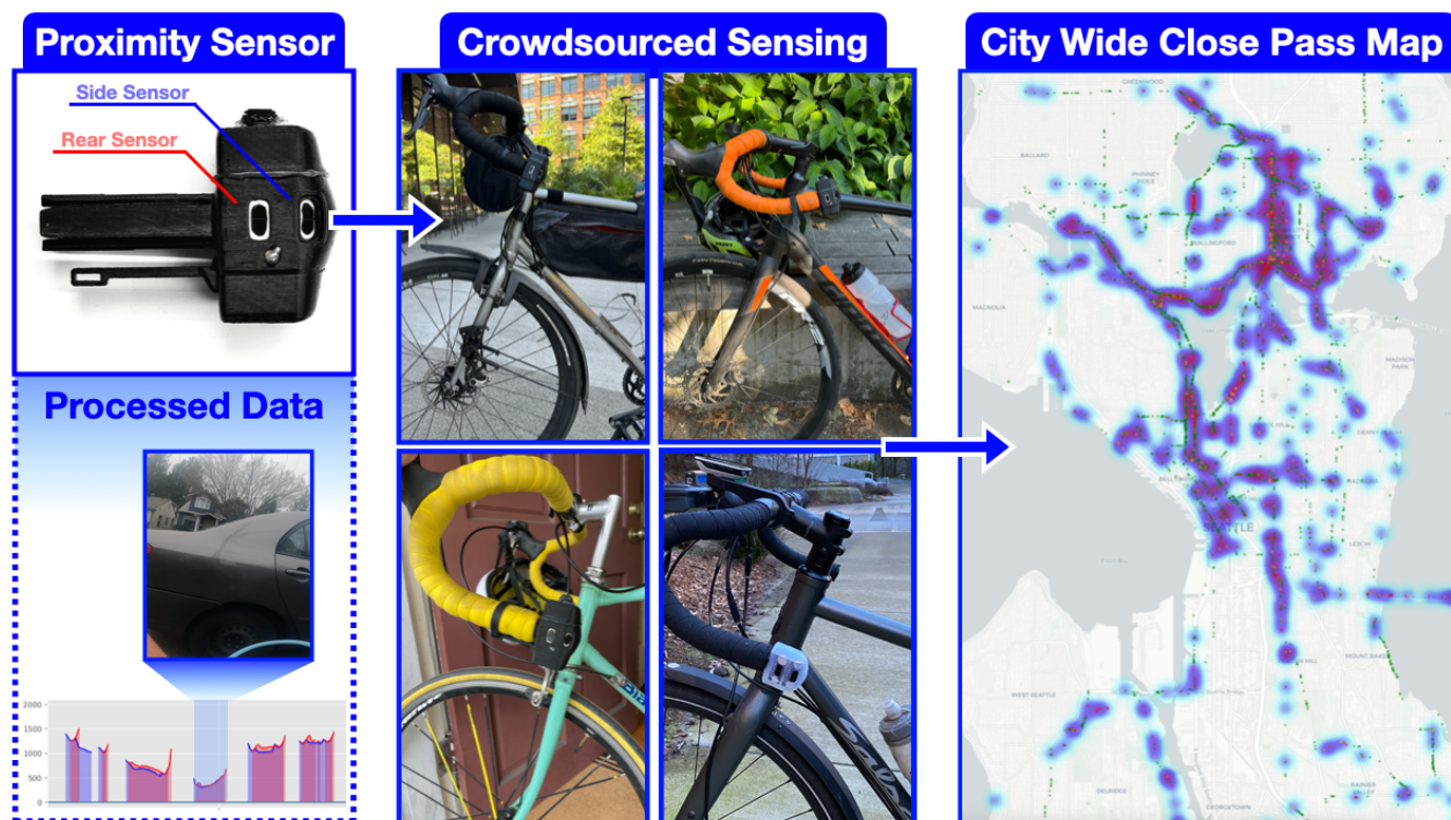
Figure 1: ProxiCycle leverages a dual proximity sensor design to retrofit and empower existing bike handlebars with the capacity to passively capture distance of passing cars during overtaking events. This data, when aggregated across many users, can provide useful insight into the safety of the road network without depending on users self-reporting.
