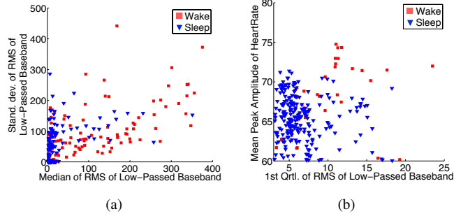
Figure 12: (a) shows a scatter plot between two frame level features: median and standard deviation of RMS energy of the low-passed ( f_c = 3Hz )baseband signal. (b) shows a scatter plot between the first quartile of RMS energy of the low-passed baseband and average amplitude of peaks of estimated heart rate.
