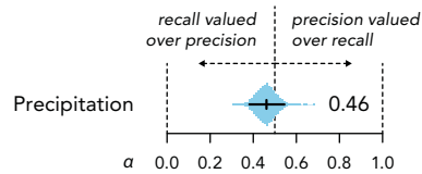
Figure 5. Posterior distributions of \alpha for precipitation prediction. Mean and 95% HDI are indicated. Note the evidence of wet bias: 82% of the distribution lies below 0.5.
