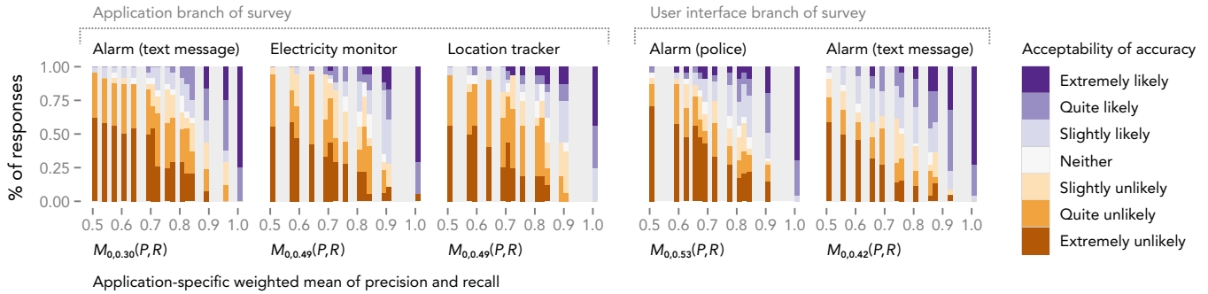
Figure 2. Acceptability of accuracy from the survey results plotted against each application’s weighted geometric mean of precision and recall from our model. Optimizing this mean has the effect of also optimizing an application’s acceptability of accuracy.
