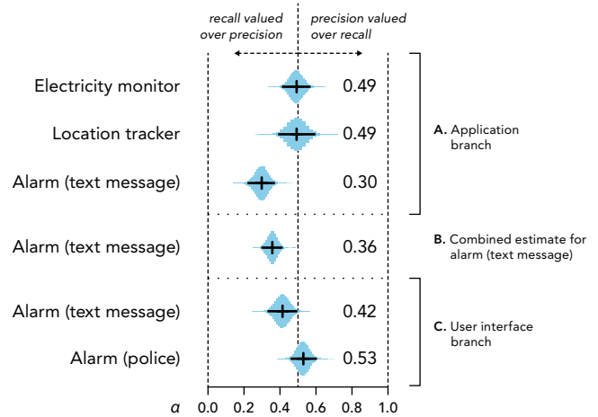
Figure 3. Posterior distributions of \alpha for both branches of the survey. Mean and 95% HDI are indicated. Note the sensitivity of our model to different preferences of precision versus recall between applications (A) and for different feedback types (C). (B) shows a more precise estimate of \alpha for alarm (text message) from a model combining both branches of the survey.
